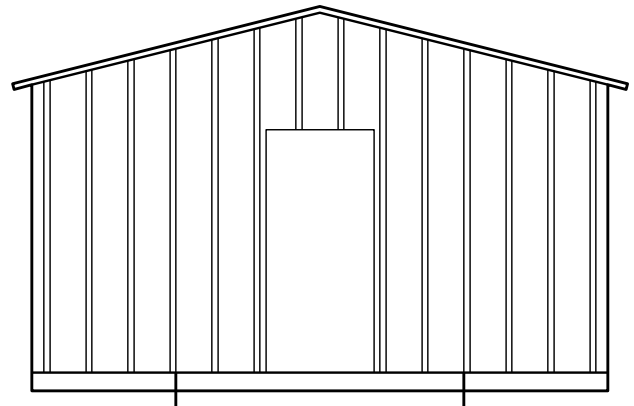
③ REAR ELEVATION \frac{3}{16}"=1'-0"
