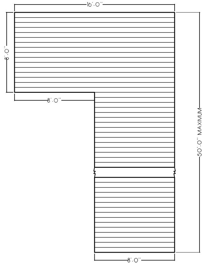
2 PIER PLAN (L) 3/16"=1'-0"
