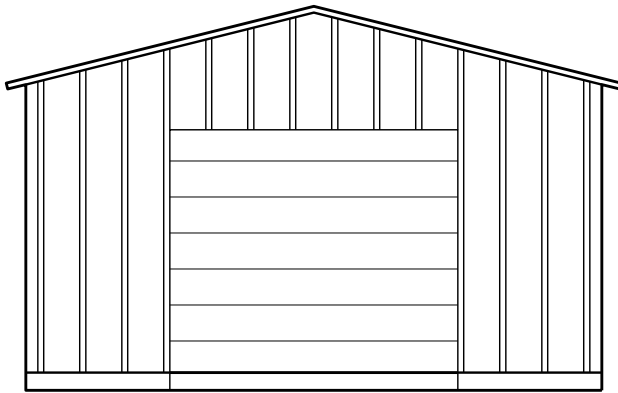
② FRONT ELEVATION \frac{3}{16}"=1'-0"
