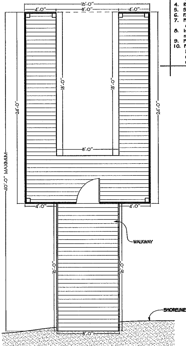
1 PLAN VIEW 3/16"=1'-0"
